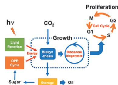
図 1 光合成細胞の基本構築 Fig. 1 Basic architect of photosynthetic cells
