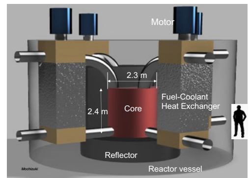
図 1 溶融塩高速炉の炉心概念 Fig. 1 Reactor Concept of Molten Salt Fast Reactor
